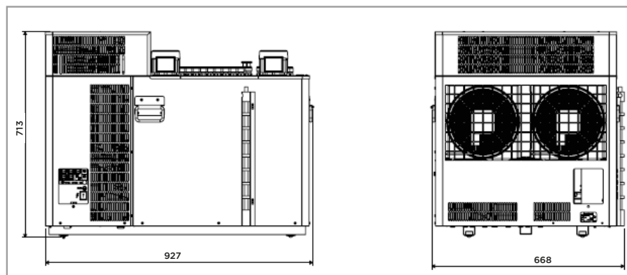
DOUBLE COOLING UNIT
