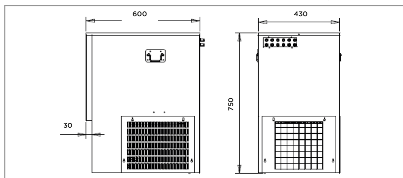
CONNESSIONI IN-OUT / IN-OUT CONNECTIONS
